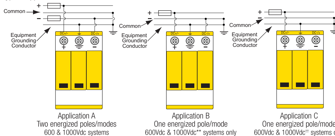
1000Vdc One energized pole/ mode mounting detail.
