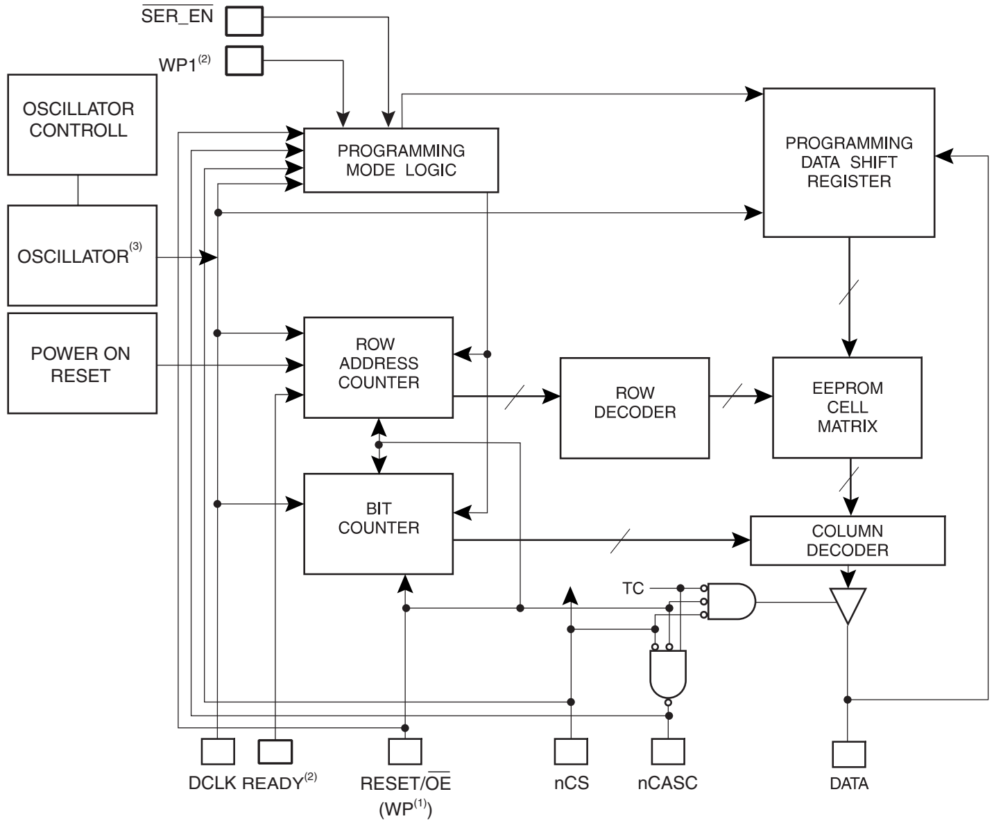
Figure 2-4. Block Diagram
