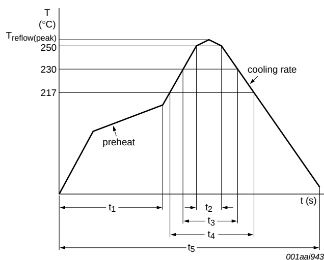
Fig 18. Pb-free solder reflow profile
