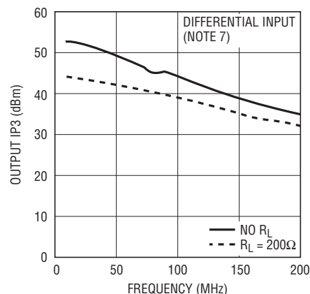
Equivalent OIP3 vs Frequency
