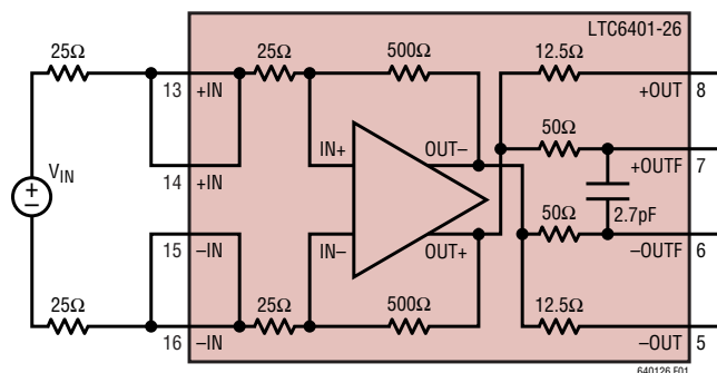
Figure 1. Input Termination for Differential 50Ω Input Impedance
