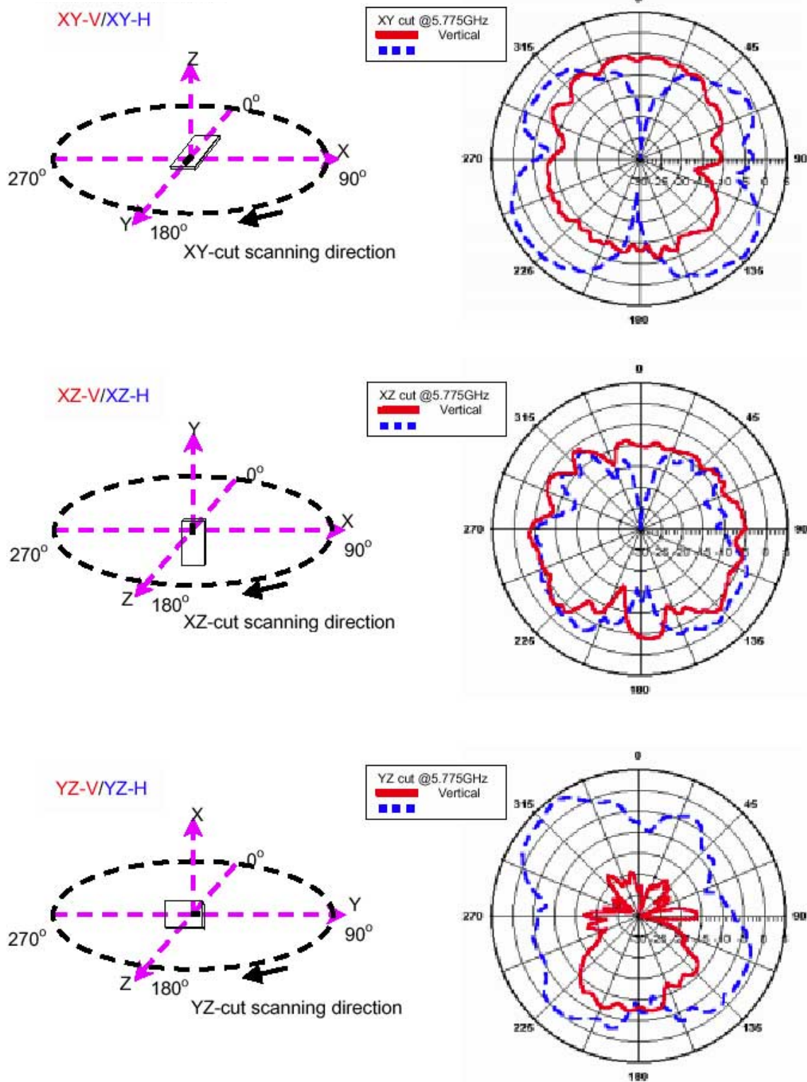
Typical Radiation Patterns for P/N 5775AT43A100
