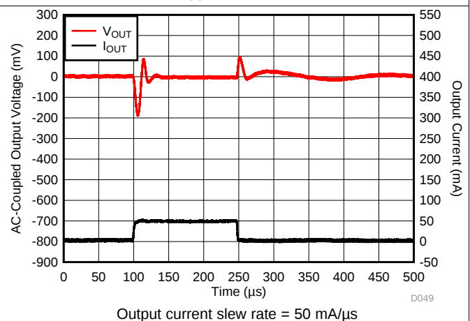
Figure 12. I_{OUT} Transient 1 mA to 50 mA
