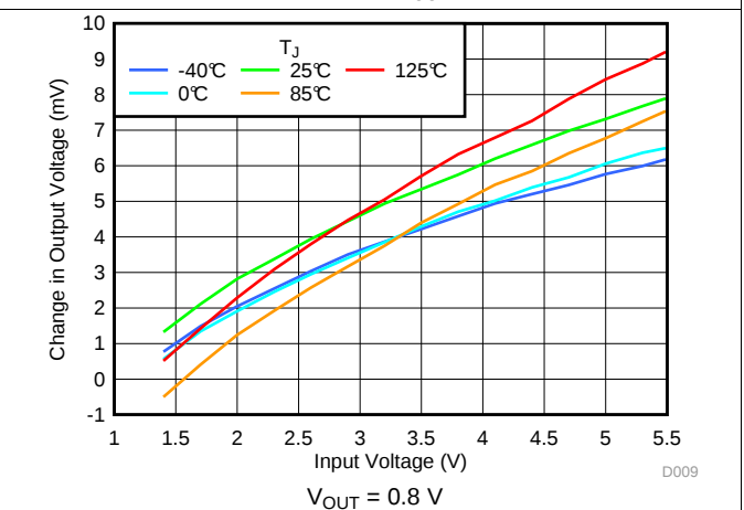
Figure 24. Line Regulation V_{IN} and Temperature
