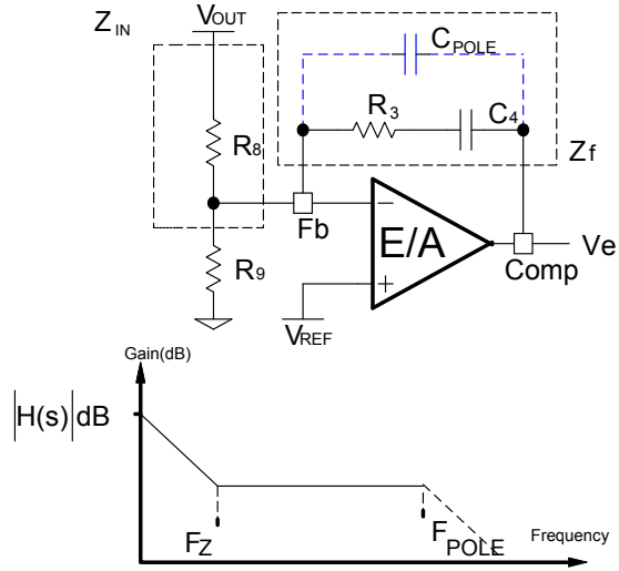
Fig. 17: Typell compensation gain network and its asymptotic gain plot
