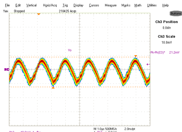
Fig. 24: Output Voltage Ripple, 25A load Ch 3 : V_{out}
