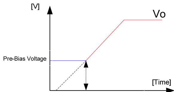
Fig. 4. Pre-Bias startup
