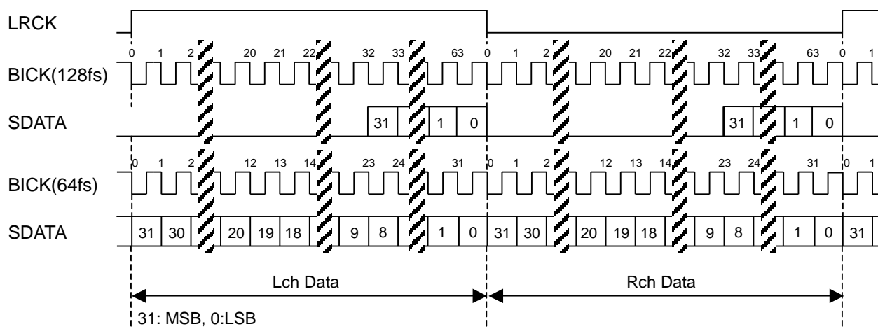
Figure 15. Mode 5 Timing
