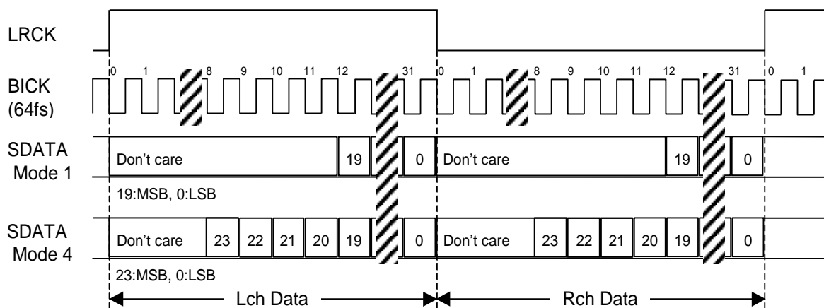
Figure 12. Mode 1/4 Timing
