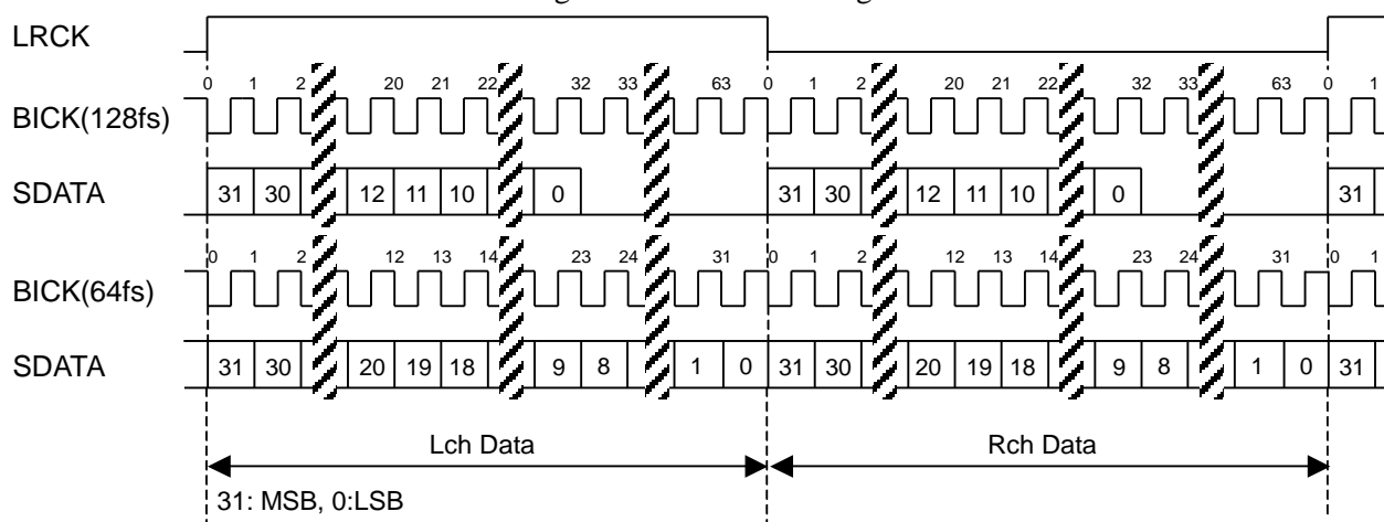
Figure 16. Mode 6 Timing
