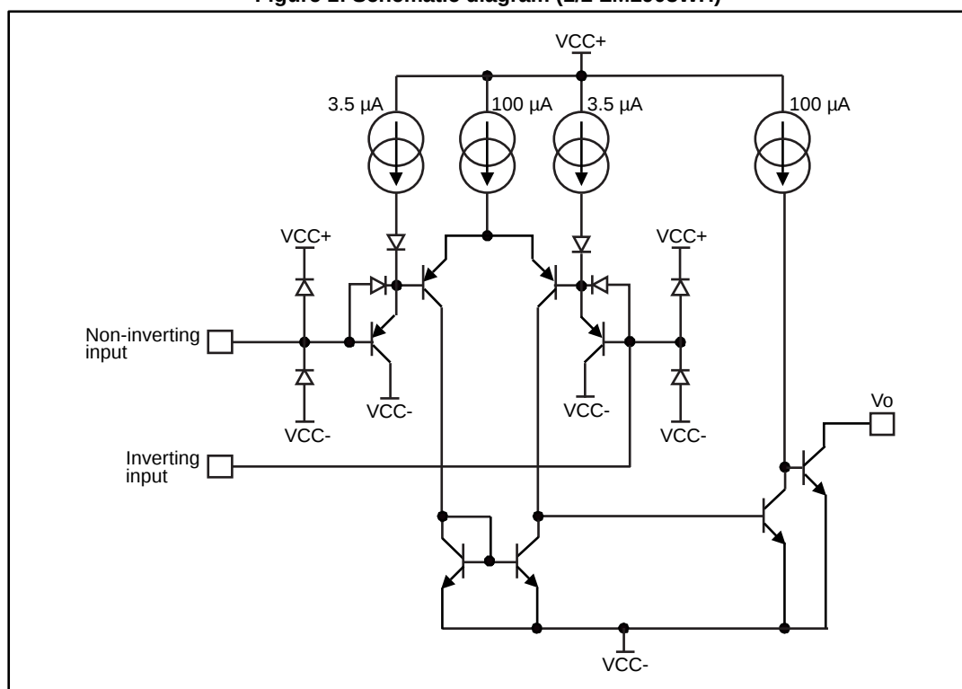
Figure 1: Schematic diagram (1/2 LM2903WH)
