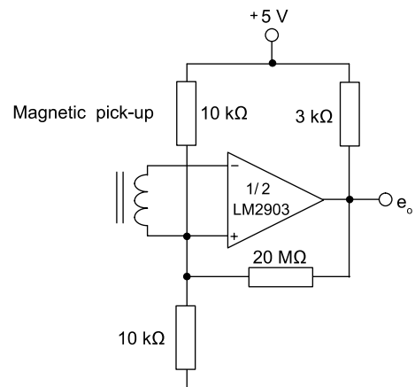
Figure 12: Transducer amplifier
