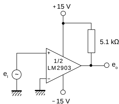
Figure 16: Split-supply applications - zero crossing detector
