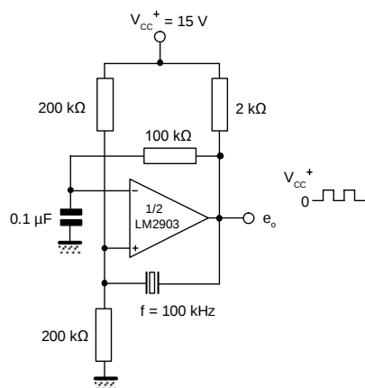
Figure 17: Crystal controlled oscillator
