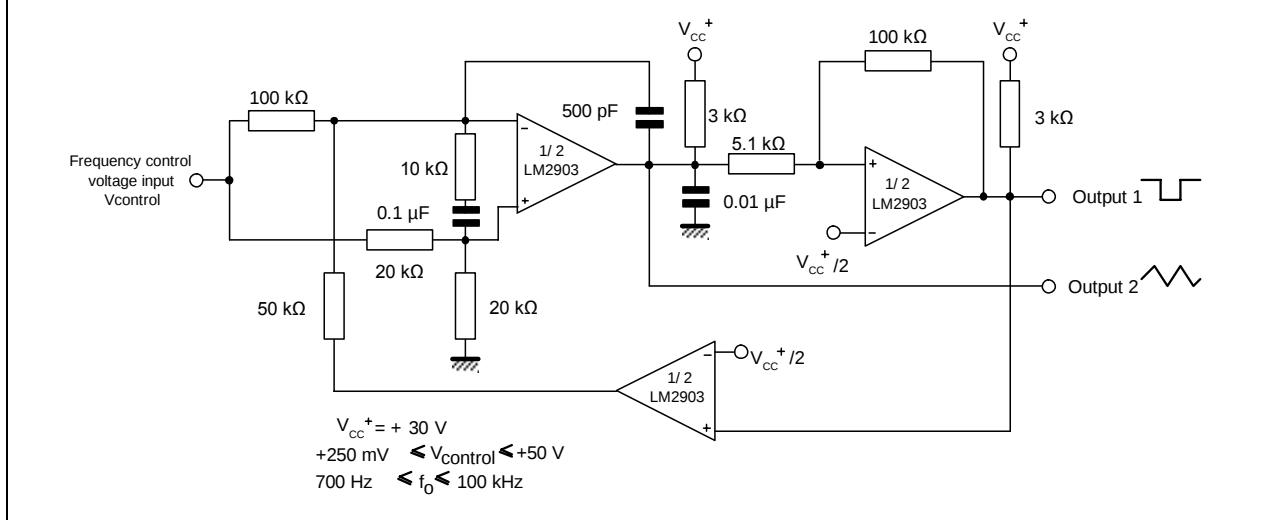
Figure 20: Two-decade high-frequency VCO
