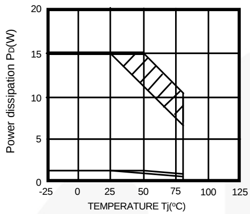
Figure 27. Power Dissipation vs. Temperature ( T_j )
