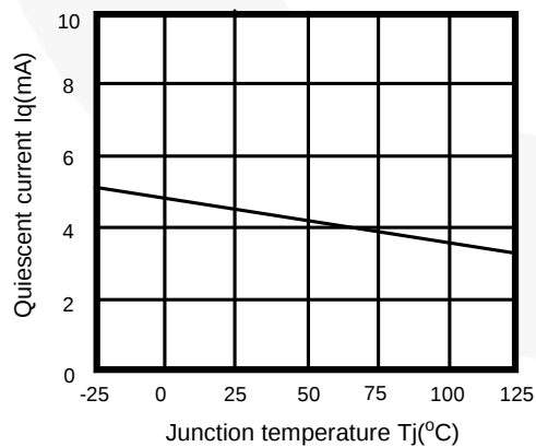
25. Quiescent Current vs. Temperature ( T_j )
