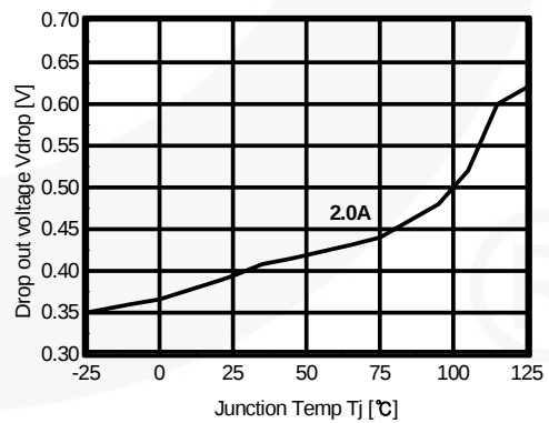
Figure 8. Dropout Voltage vs. Junction Temperature
