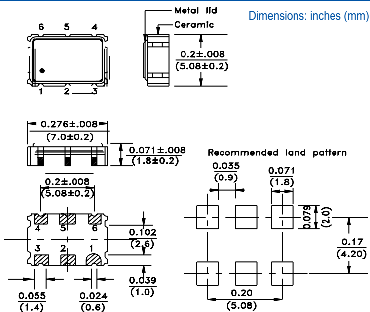
Bottom view
