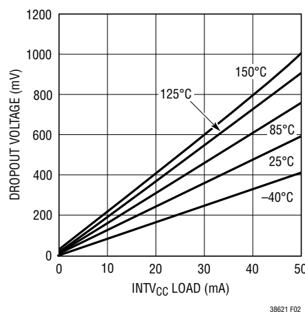
Figure 2. INTV_{CC} LDO Dropout Voltage vs Current
