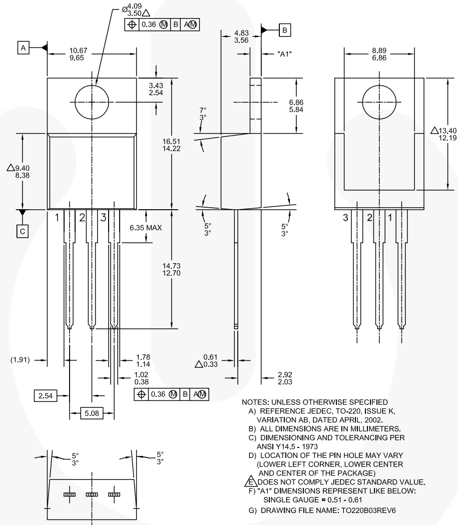
Figure 13. TO220, MOLDED, 3-LEAD, JEDEC, VARIATION AB
