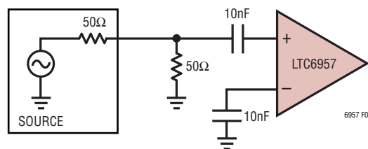
Figure 3. Single-Ended 50Ω Input Source
