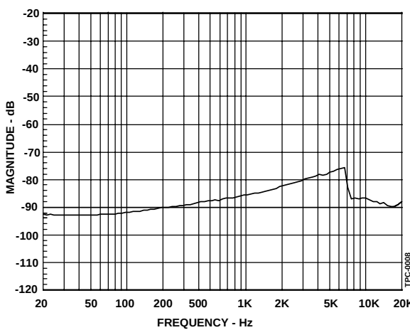
Figure 14. THD+N vs Distortion, 1W into a 6Ω Load
