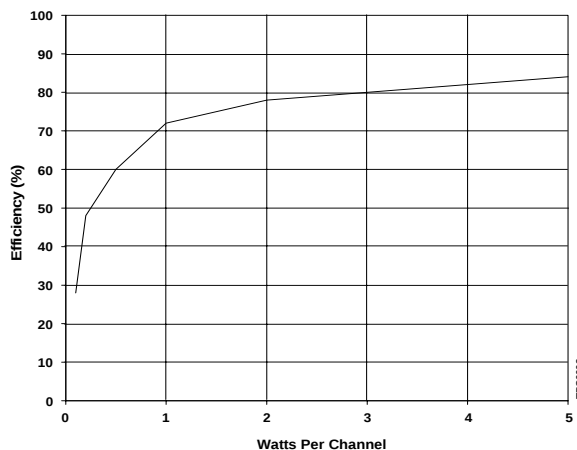
Figure 13. Efficiency vs Power
