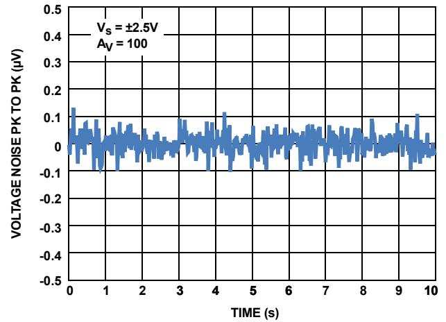
FIGURE 68. OP AMP 0.1Hz TO 10Hz PEAK-TO-PEAK VOLTAGE NOISE
