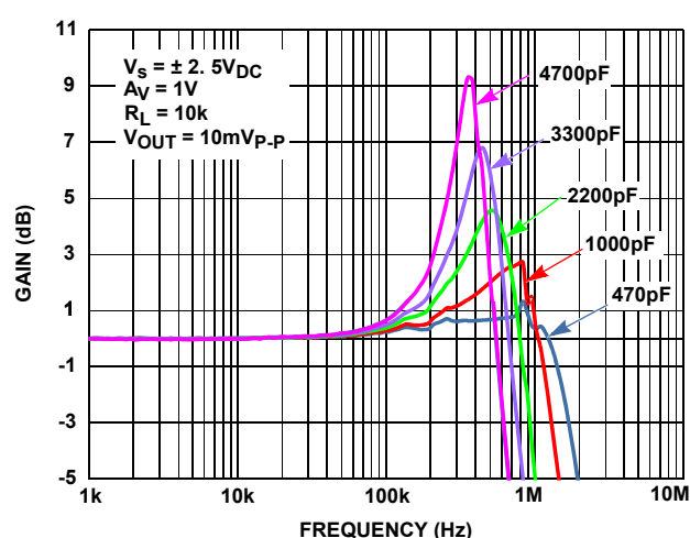
FIGURE 40. PGIA GAIN vs FREQUENCY vs CL, ISL2863x
