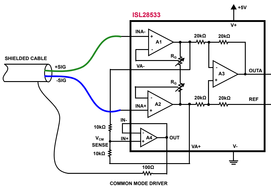
FIGURE 78. APPLICATION CIRCUIT: ACTIVE SHIELD DRIVER
