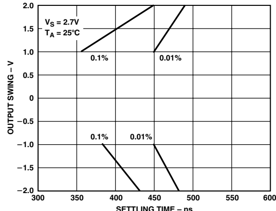
TPC 48. Output Swing vs. Settling Time
