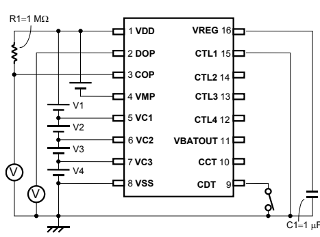
Test circuit 4
