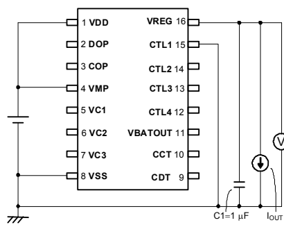
Test circuit 2
