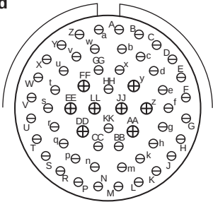
front face of pin inserts illustrated
