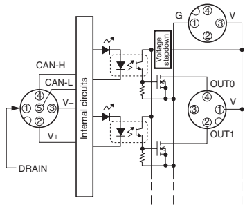
DRT2-WD16CL (NPN)
