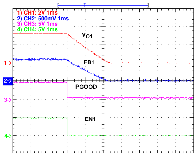
FIGURE 10. ENABLE CONTROL, EN1 = \text{LOW} , V_{IN} = 12V , V_{O1} = 3.3V , I_{O1} = 5A
