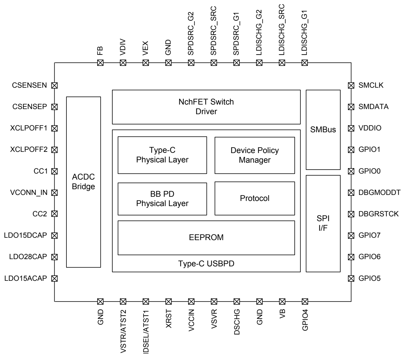
Figure 3-1 Block Diagram
