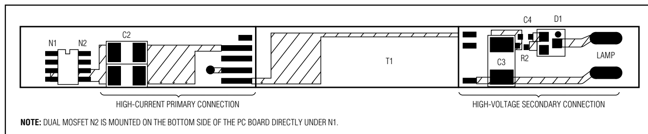
Figure 9. High-Voltage Components Layout Example
