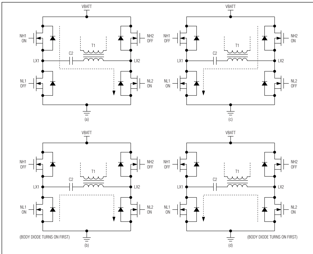
Figure 3. Resonant Operation
