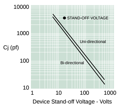
Figure 3 - Capacitance vs. Stand-off Voltage
