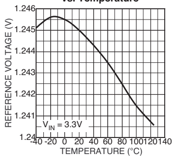
Error Amp Reference Voltage vs. Temperature
