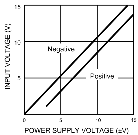
Figure 12: Input voltage range
