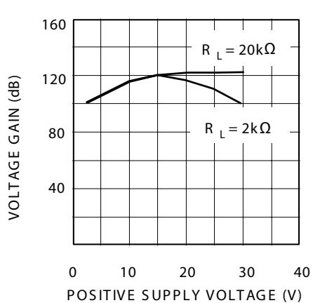
Figure 13: Voltage gain
