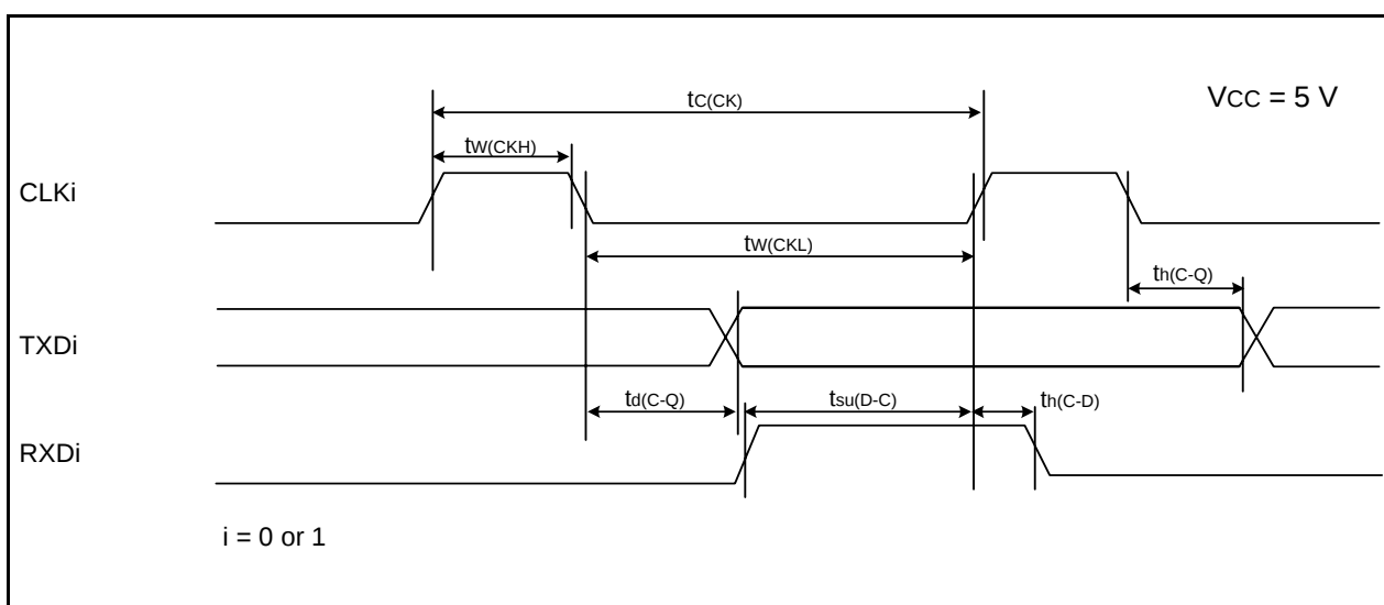
Figure 5.29 Serial Interface Timing Diagram when V_{CC} = 5 \text{ V}
