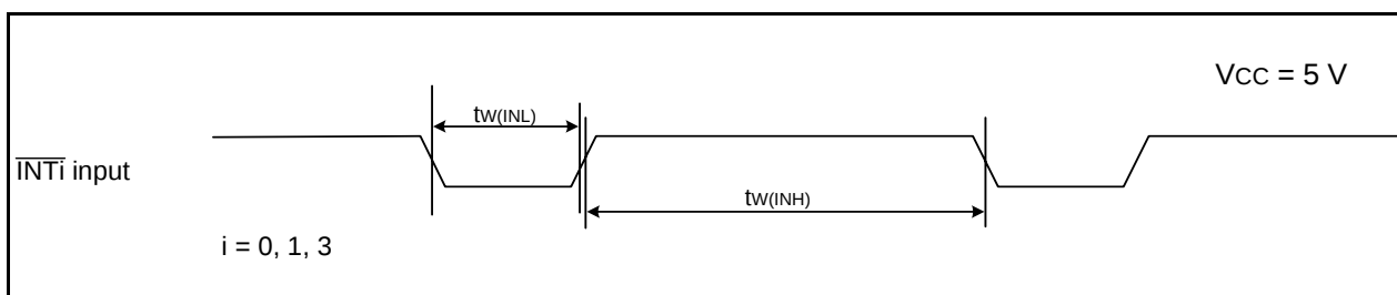
Figure 5.30 External Interrupt \overline{INTi} Input Timing Diagram when V_{CC} = 5 \text{ V}
