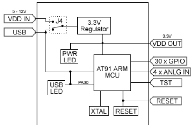
ECIO ARM Block Diagram
