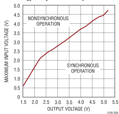
V_{\text{IN}} for Synchronous Operation
