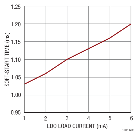
LDO Soft-Start Duration vs LDO Load
