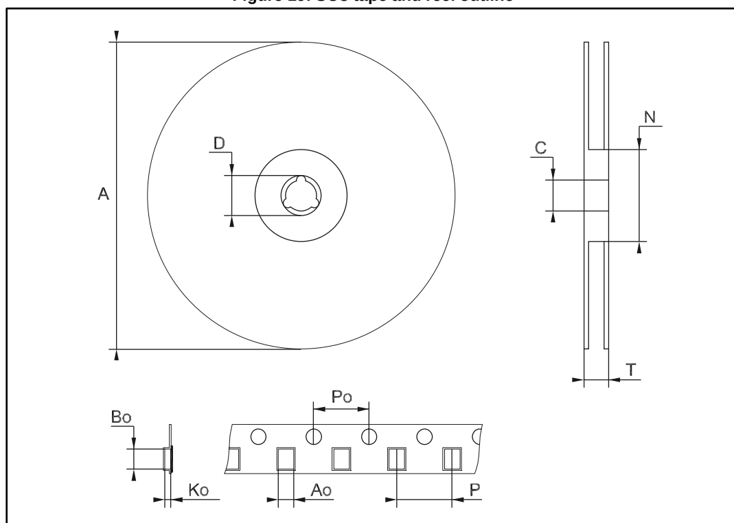
Figure 19: SO8 tape and reel outline
