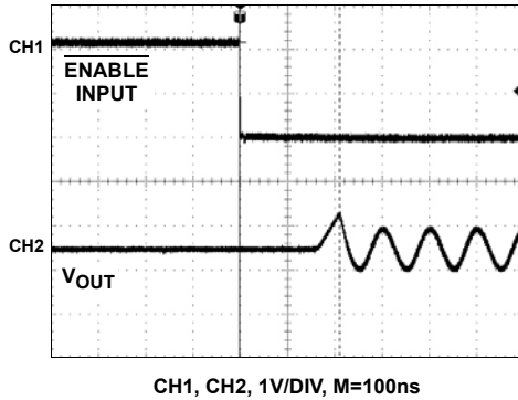
FIGURE 27. ENABLED RESPONSES
