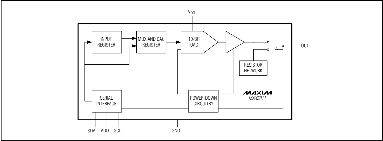
Functional Diagram
