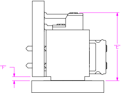
FIG 4 SFM-D-SM MATED WITH TFM-DH
