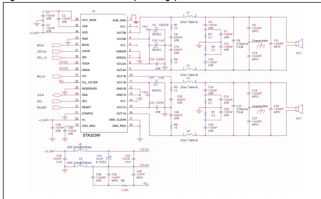
Figure 6. Power schematic for 2 (full-bridge) channels
