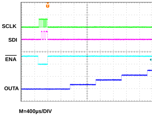
FIGURE 3. LARGE SIGNAL RESPONSE (RISING FROM 0V TO 8V)
