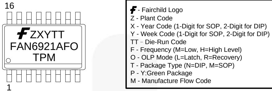
Figure 3. Marking Diagram
