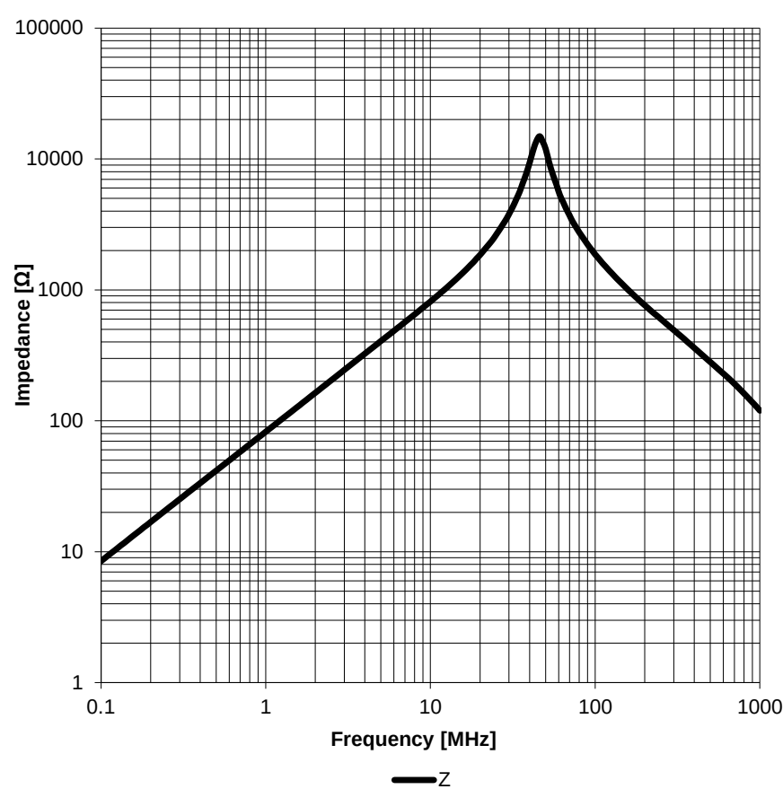
Typical Impedance Characteristics:
