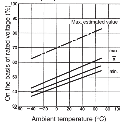
Ambient Temperature vs. Must Set or Must Reset Voltage G6KU-2G (F/P)-Y
