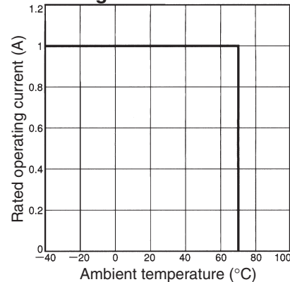
Ambient Temperature vs. Switching Current
