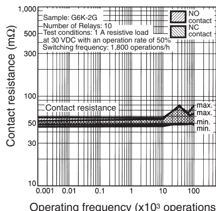
Electrical Service Life (Contact Resistance) (See note.) G6K-2G (F/P), G6K-2G (F/P)-Y
