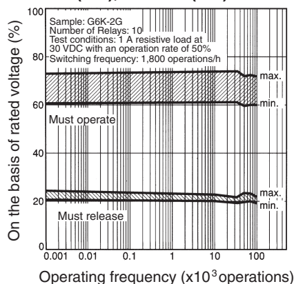
Electrical Service Life (with Must Operate and Must Release Voltage) (See note.) G6K-2G (F/P), G6K-2G (F/P)-Y
