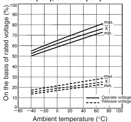
Ambient Temperature vs. Must Operate or Must Release Voltage G6K-2G (F/P), G6K-2G (F/P)-Y
