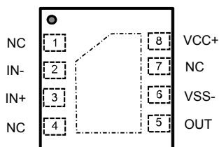
DFN8 2 x 2
