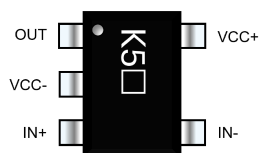
Figure 1. Pin connection SC70-5 and SOT23-5 (top view)
