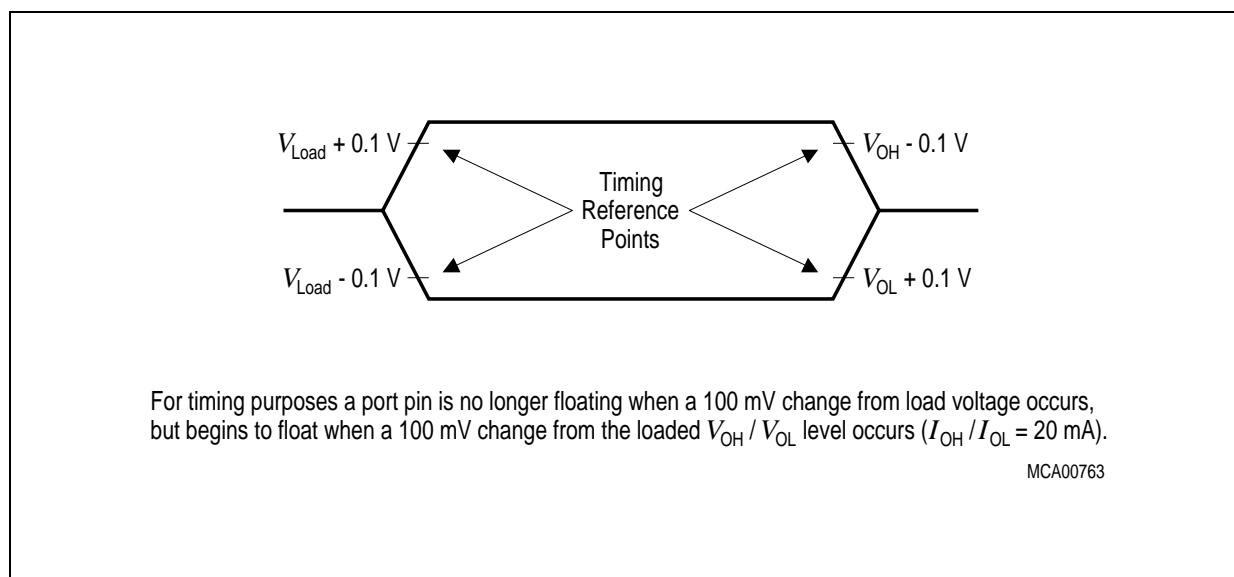
Figure 19 Float Waveforms
