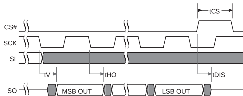
Figure 6.11 SPI Single Bit Output Timing
