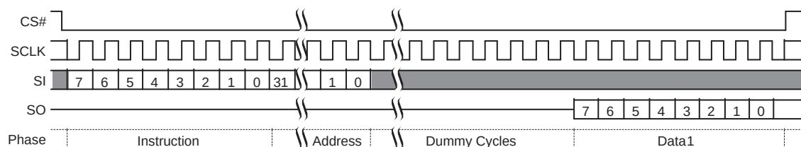
Figure 4.7 Single Bit Wide I/O Command with Latency
