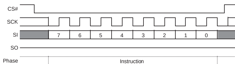
Figure 10.72 Software Reset Command Sequence
