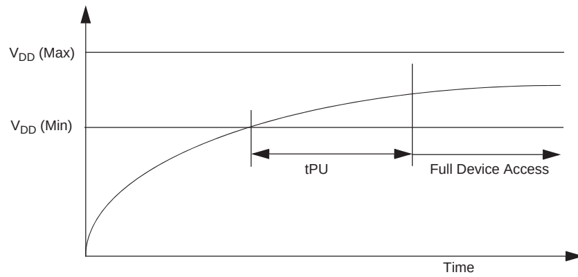
Figure 5.3 Power-Up
