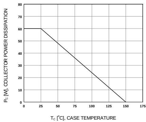
Figure 11. Power Derating
