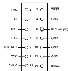
14-pin TI-style JTAG pinout
