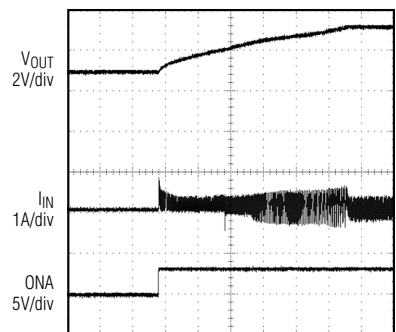
STARTUP WAVEFORMS USING SOFT-START
