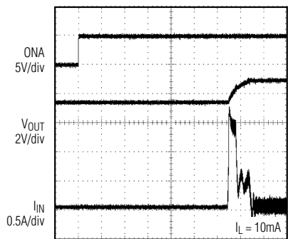
POWER-ON DELAY
