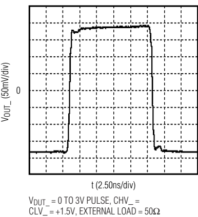
COMPARATOR DIFFERENTIAL OUTPUT RESPONSE (MAX9967_LCCQ)
