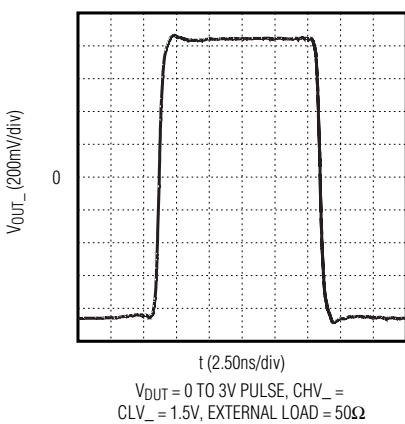
COMPARATOR DIFFERENTIAL OUTPUT RESPONSE (MAX9967_MCCQ)
