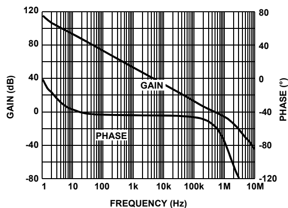
FIGURE 5. A_{VOL} vs FREQUENCY @ 100kΩ LOAD
