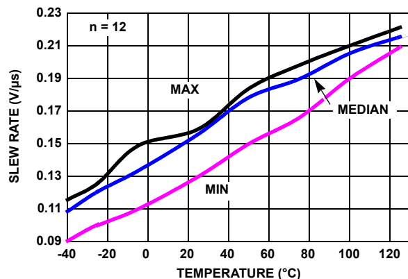
FIGURE 55. ISL28176 + SLEW RATE vs TEMPERATURE, V_{OUT} = \pm 1.5V , A_V = +2
