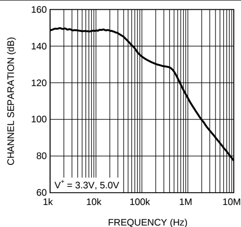
Figure 28. Channel Separation vs Frequency
