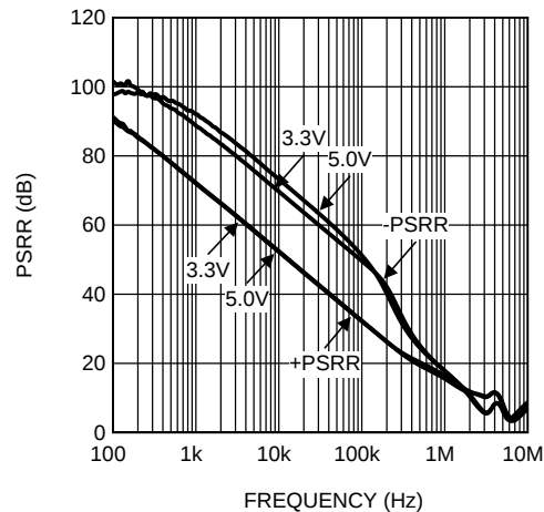
Figure 26. PSRR vs Frequency
