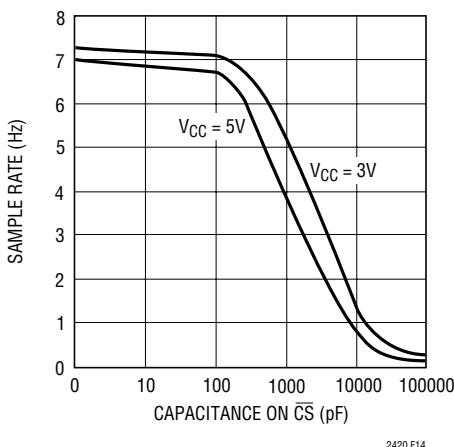
Figure 14. \overline{\text{CS}} Capacitance vs Output Rate
