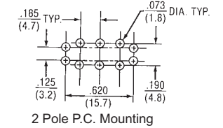
2 Pole P.C. Mounting
