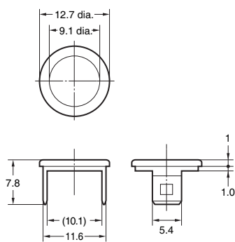
Flange (Round) A3A-25
